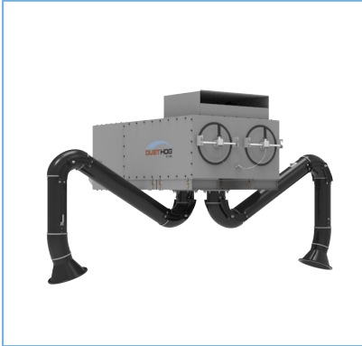
Wall-mount weld fume collector are ideal for capturing submicron weld fume and smoke from a fixed workspace. Available with one or two extraction arms.
